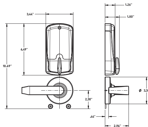
Mortise Deadbolt
