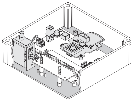
RLBD Installed in PIM400-TD2
