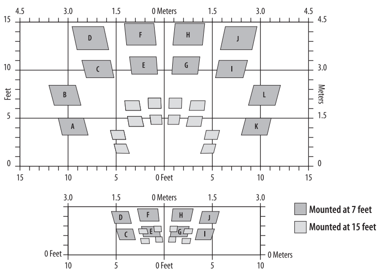
Standard Pattern Shown wall mounted, angled 14° down.
